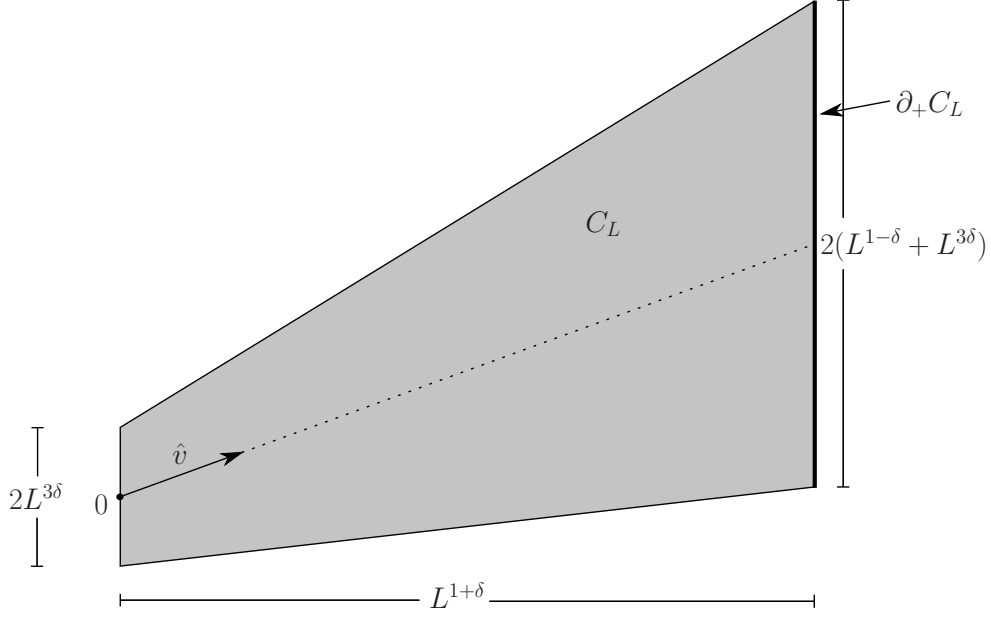
Figure 3: The set C_L and its boundary part \partial_+ C_L .
