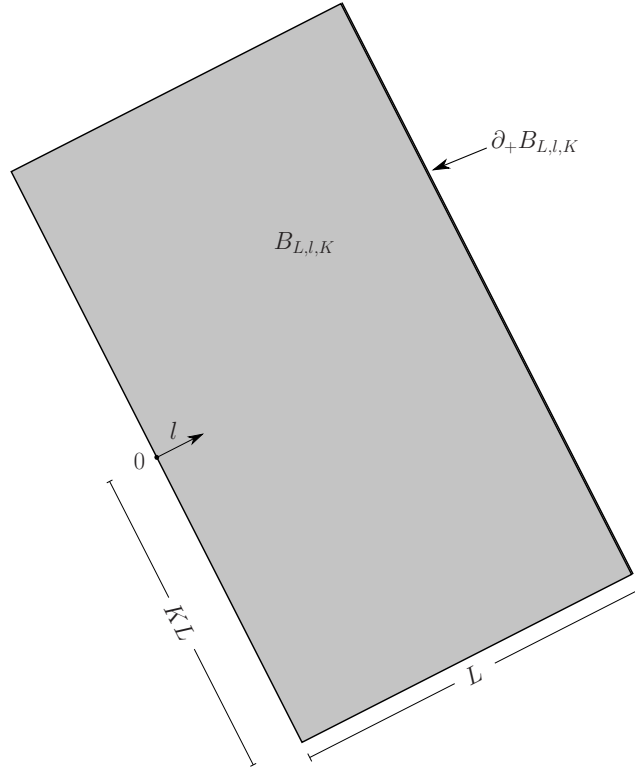
Figure 2: The set B_{L,l,K} and its boundary part \partial_+ B_{L,l,K} .
