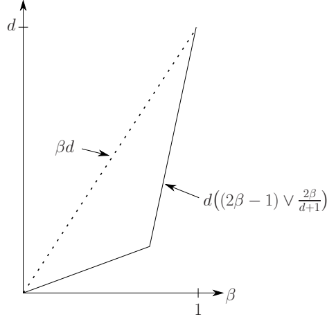
Figure 1: Sketch of the known and conjectured bounds for \alpha .
