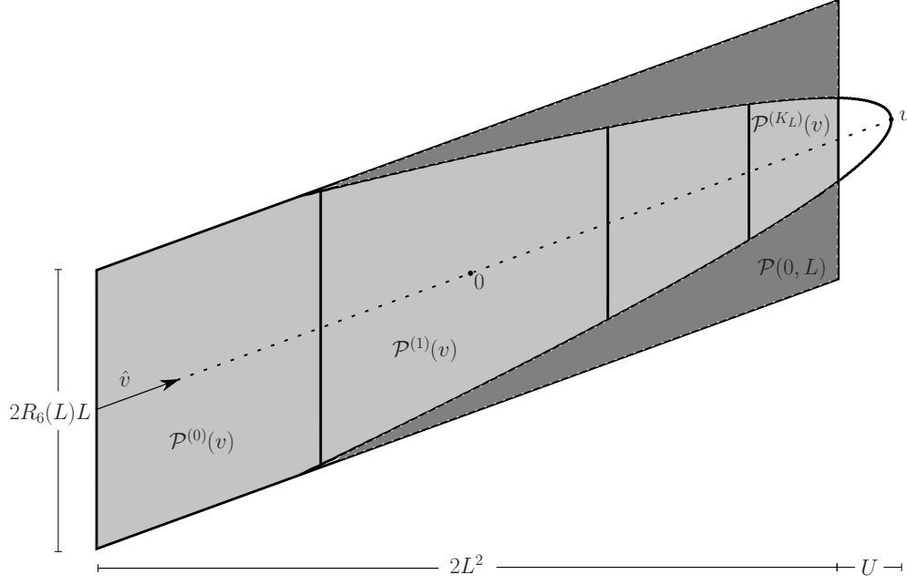
Figure 5: The sets \mathcal{P}^{(k)}(v) contained in \mathcal{P}(0, L) .
