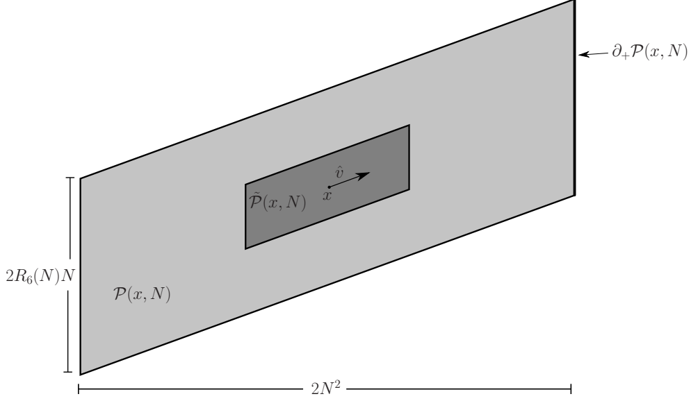
Figure 4: The set \mathcal{P}(x, N) and its right boundary part \partial_+\mathcal{P}(x, N) as well as its middle third \tilde{\mathcal{P}}(x, N) .
