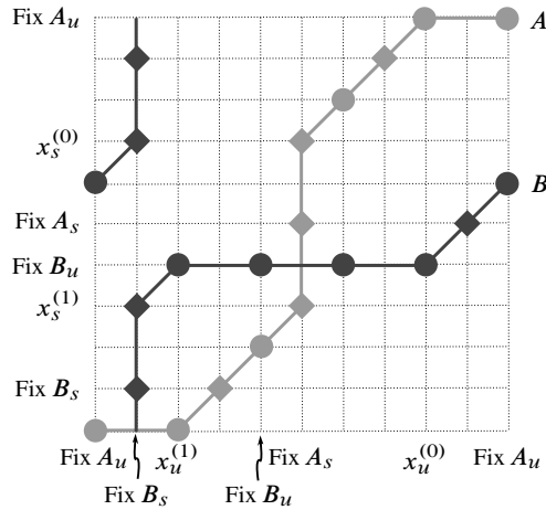
Figure 14. The correspondences A and B for p/q = 2/5 .
