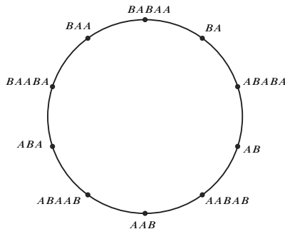
Figure 6. Order on O(2/5) \sqcup O(1/3) \sqcup O(1/2) .
