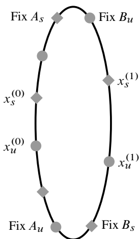
Figure 13. The pair of multicones M for p/q = 2/5 .
