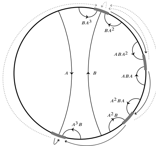
Figure 1. Example of a uniformly hyperbolic pair (A, B) and a multicone. Outer arrows indicate the action of A and B in the components of the multicone. Inner arrows indicate stable and unstable directions of A, B , and some of their products.
