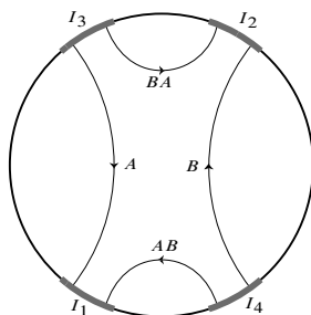
Figure 5. Group-hyperbolicity of the free component.
