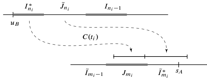
Figure 10. Proof of (34).
