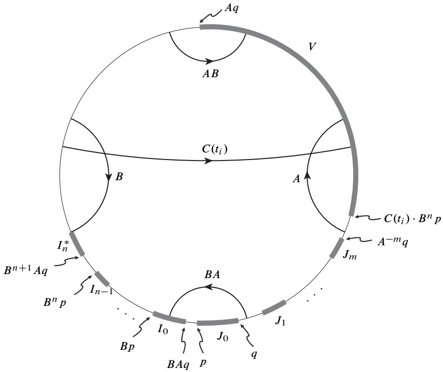
Figure 9. A “non-strict” multicone for (A, B, C(t_i)) .
