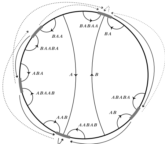
Figure 2. Another example of a uniformly hyperbolic pair (A, B) .
