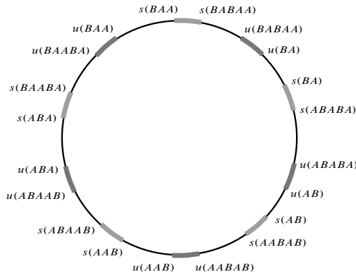
Figure 7. The intervals I_\omega^u, I_s^\omega for p/q = 2/5 .
