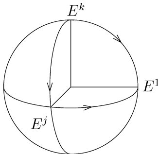
Fig. 1. Uniform projective hyperbolicity.
